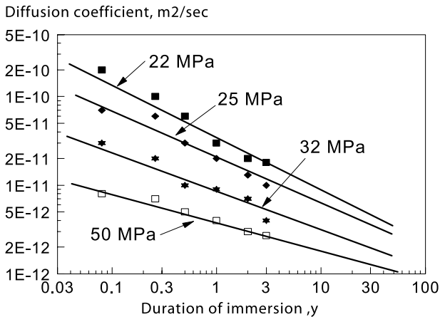
Figure 2: Observed variation of D for concretes of different grades after immersion in seawater.
