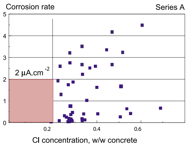
Figure 3: Corrosion rate of steel vs Cl concentration in different concretes and covers
